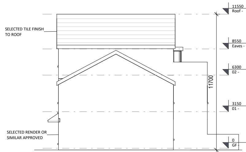
4 Side Elevation 02 1 : 200
